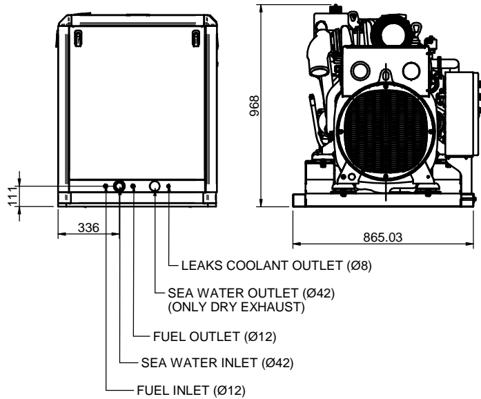
VIEW A
