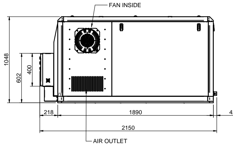
VIEW C
